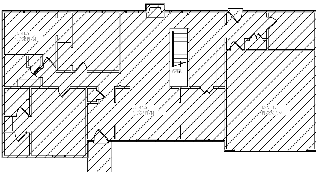
EXISTING FLOOR PLAN
