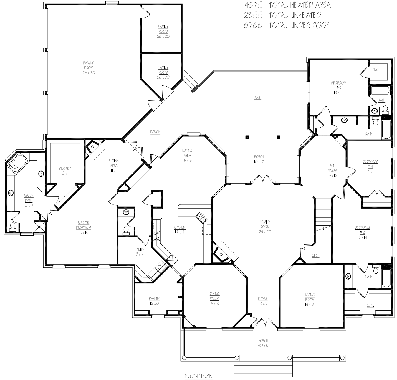
FLOOR PLAN
