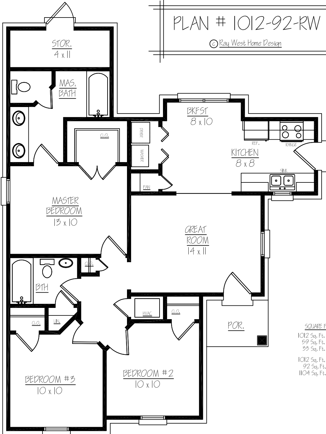
FLOOR PLAN
